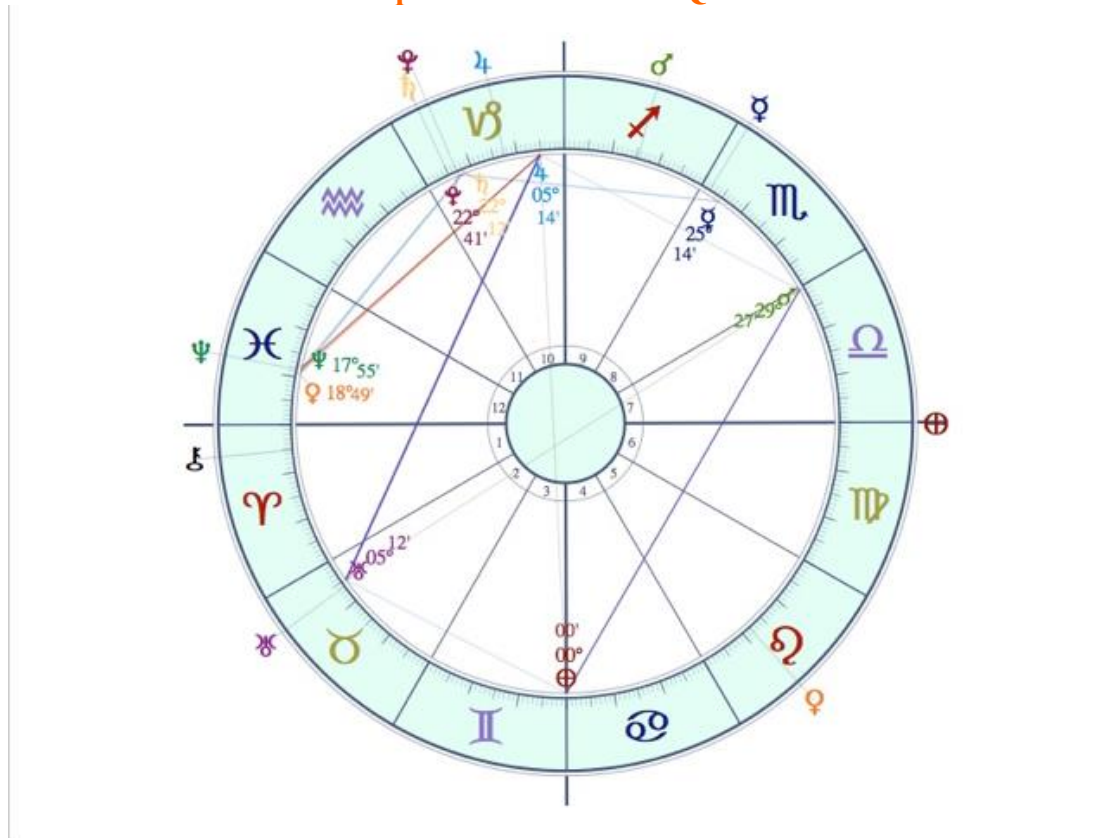
Inner Wheel: 22 December 2019 h 4.21 GMT – Outer Wheel: 20 March 2020 h 3.50
