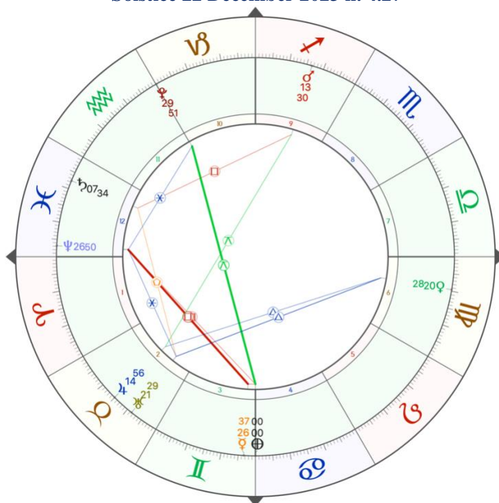
Solstice 22 December 2023 h. 4.27
